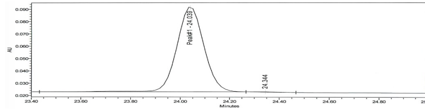
HPLC-UV Chromatogram
